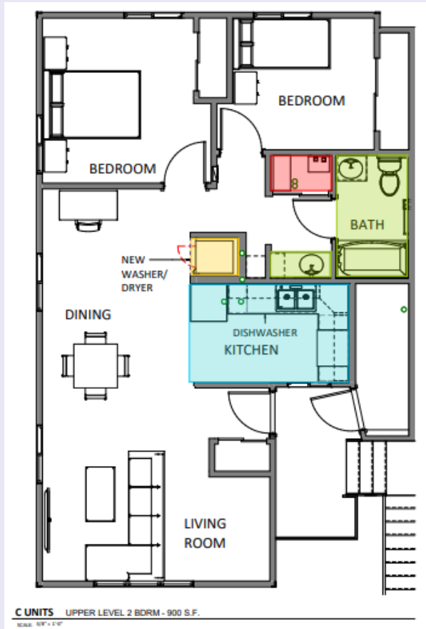
Villages on Swallow: 2 Bedroom— updated floor plan—C Units 900 Sq Ft
